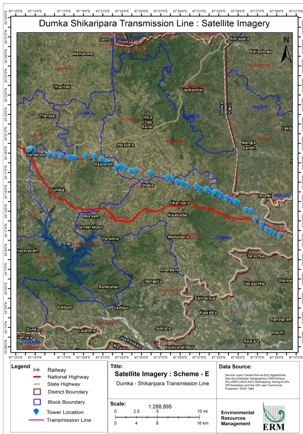
Figure 3.3 Dumka- Shikaripara TL Alignment on Satellite Imagery
