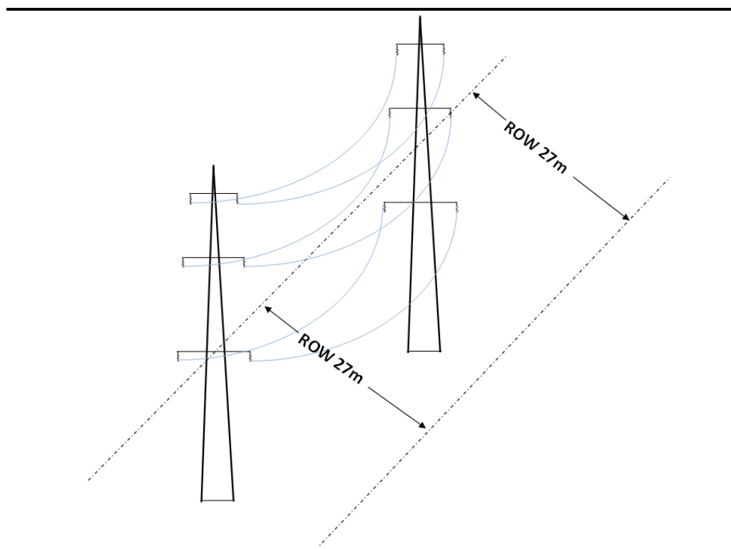
Figure 3.4 Right of Way for 132 KV Transmission Line
